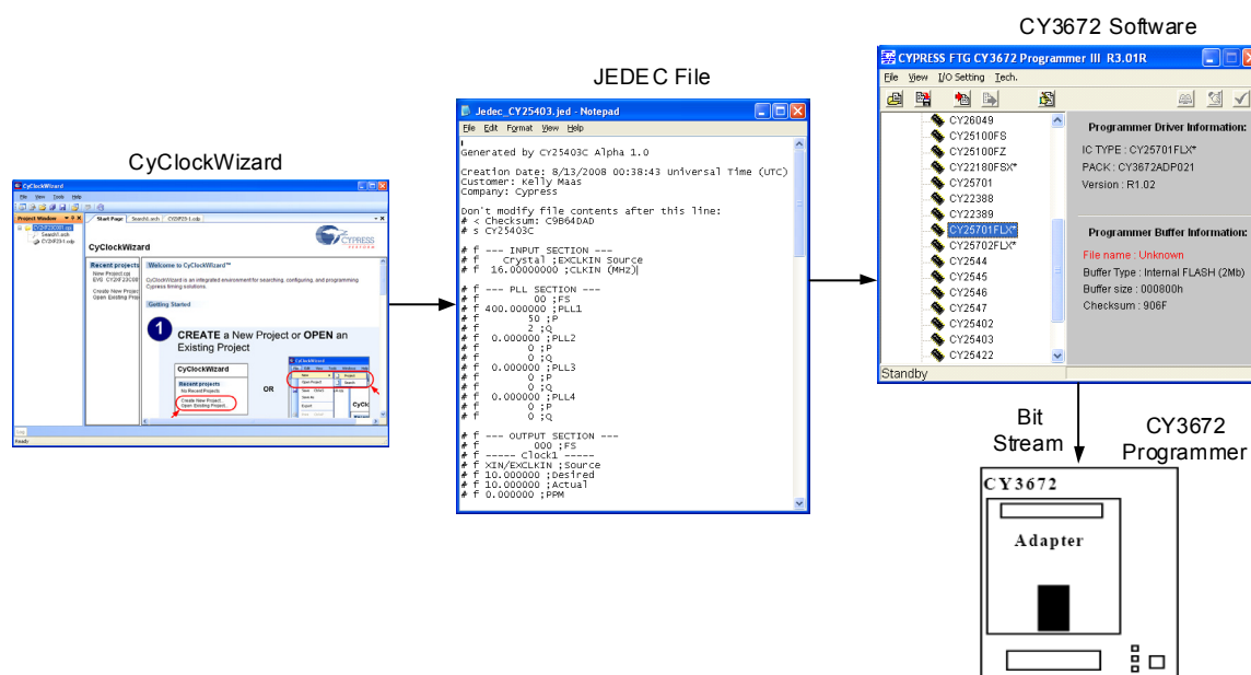
Figure 1. Programming Procedure
